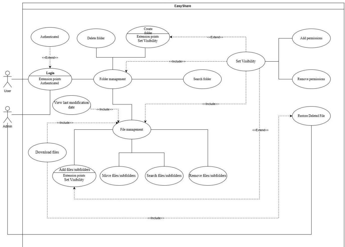
Diagram 1: Use case diagram
